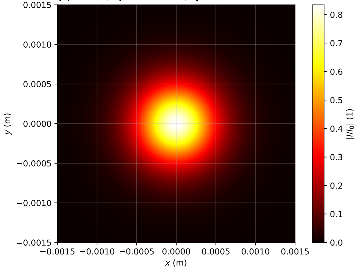
Intensity profile I(x, y, z = 3.025m)/I_0 , \text{Pin}=0.7\text{Pcr} , artificial time
